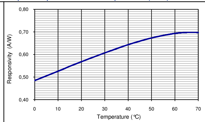
Responsivity as funtion of temperature (10 V)
